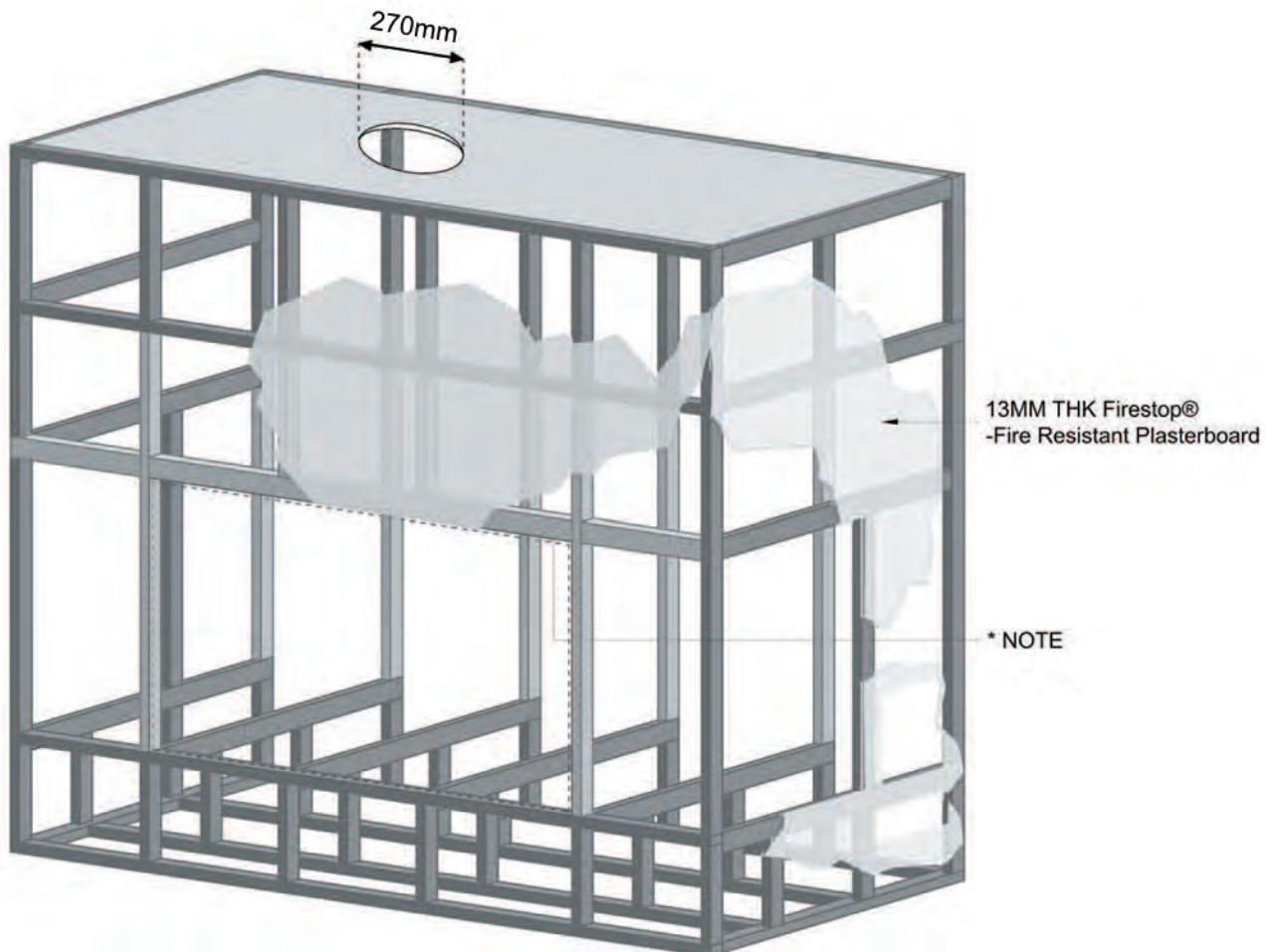
Figure 1.7 (Cladding Material)
